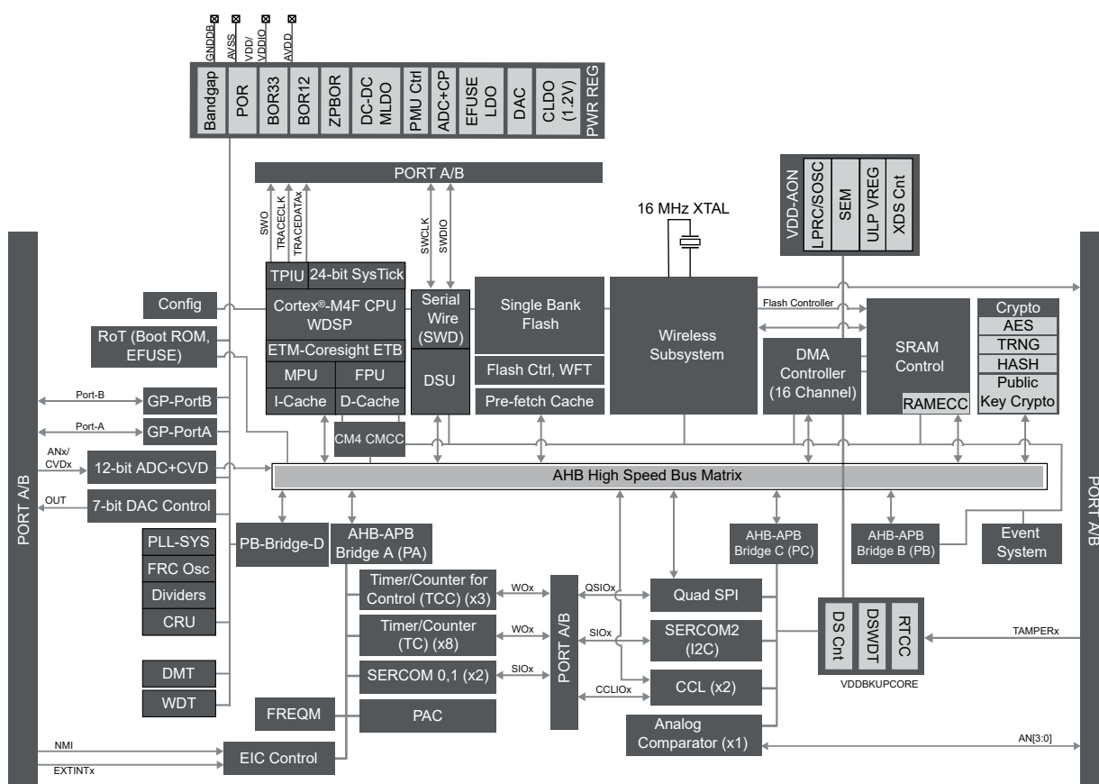
Figure 3-1. PIC32CX-BZ3 SoC Block Diagram
