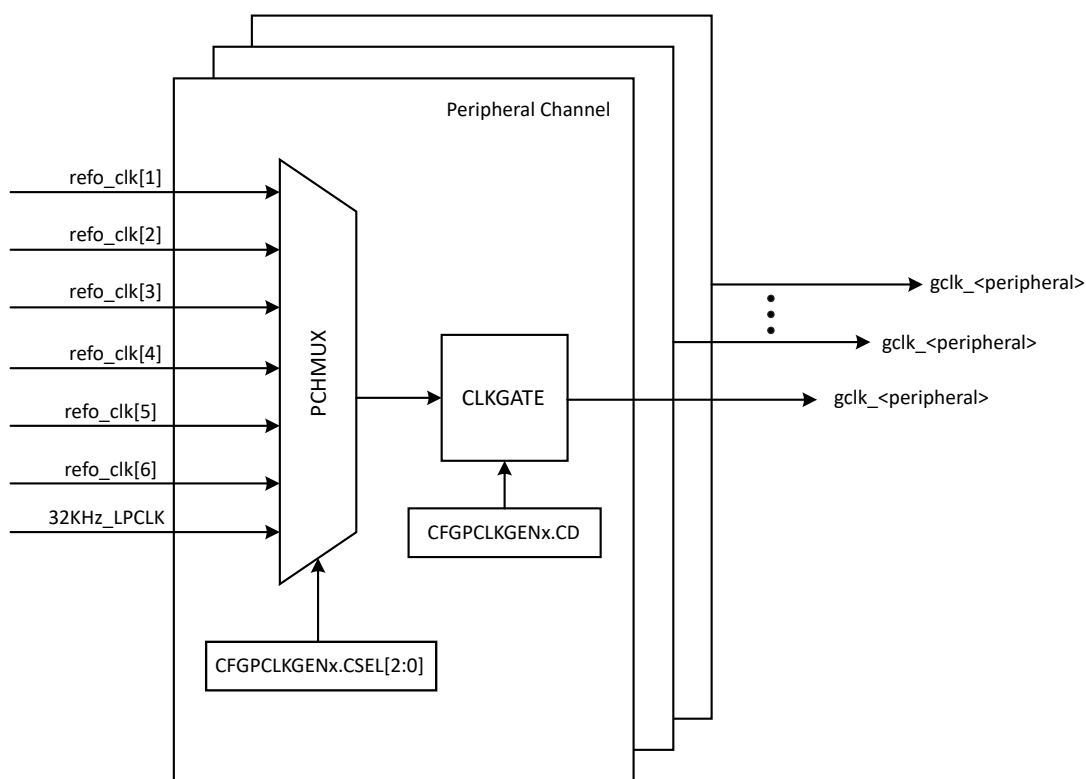
Figure 17-3. Peripheral Clock Generation (GCLK)
