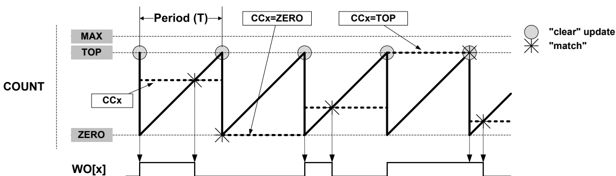
Figure 41-6. Single-Slope PWM Operation
