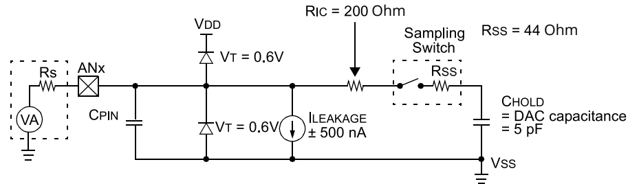
Figure 36-12. 12-bit ADC Analog Input Model
