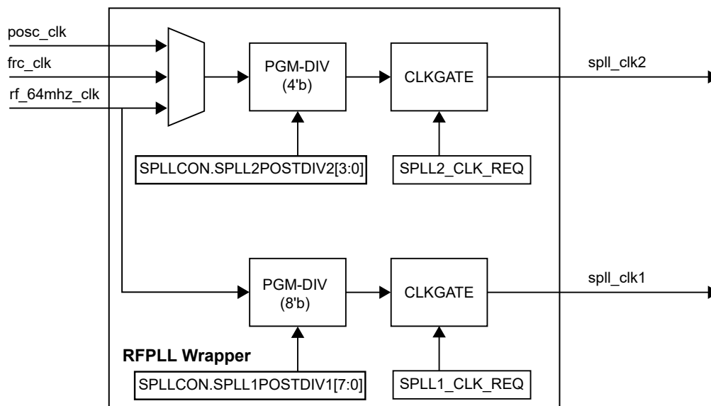
Figure 17-2. RFPLL Wrapper
