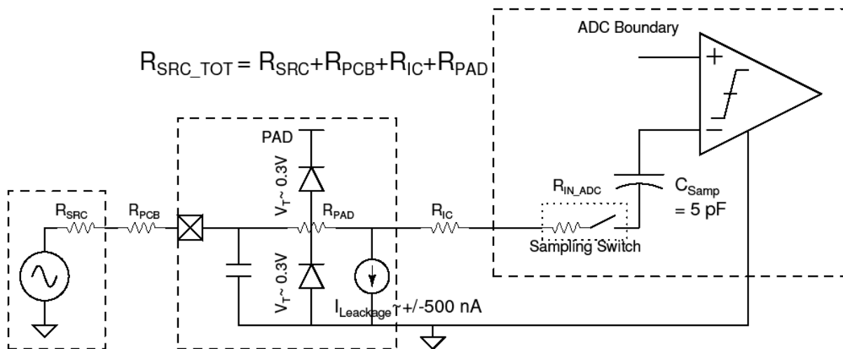
Figure 36-13. Simplified Analog Input Model
