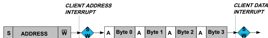
Figure 34-14. 32-Bit Extension Client Operation
