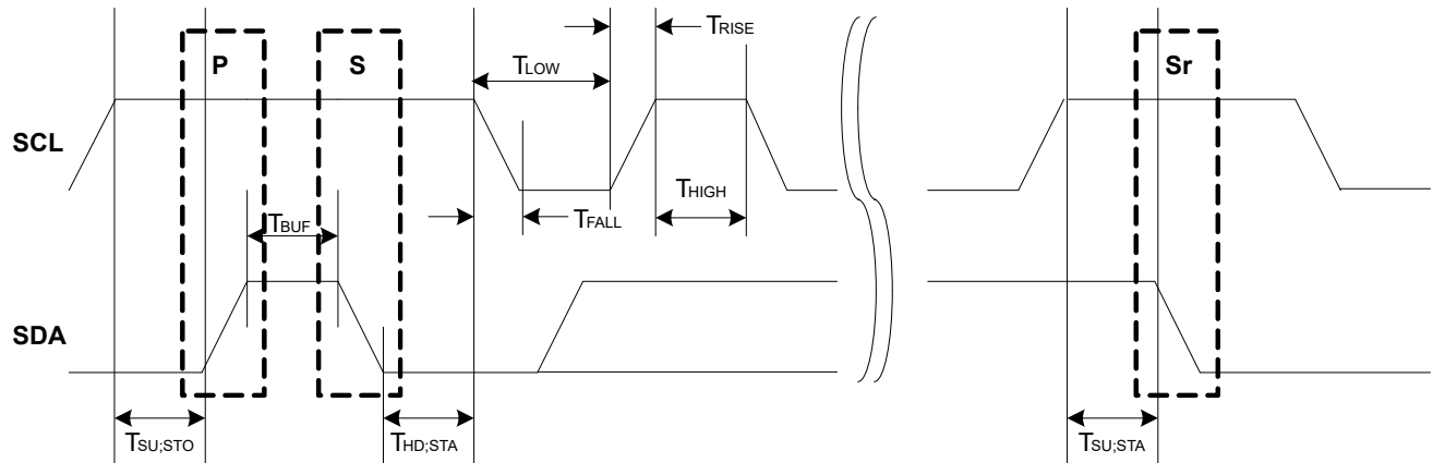
Figure 34-7. SCL Timing
