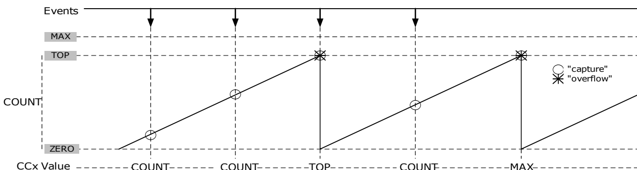
Figure 40-15. Time Stamp
