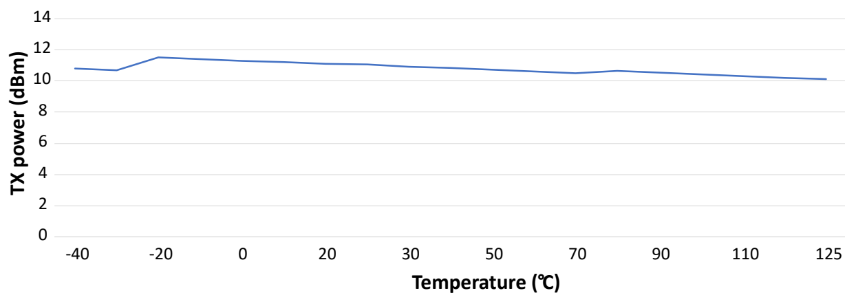
Figure 43-29. Zigbee Transmit Power vs. Temperature
