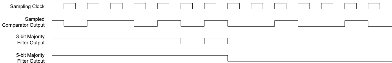
Figure 38-6. Continuous Mode Filtering
