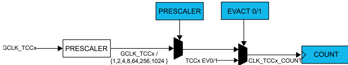
Figure 41-2. Prescaler
