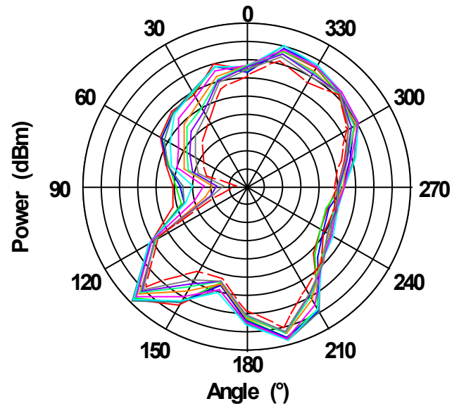
Figure 4-15. WBZ351 Antenna Radiation Pattern when \Theta = 90^\circ
